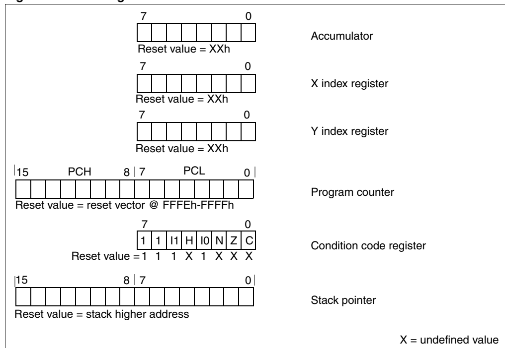
Figure 7. CPU registers
