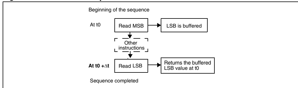
Figure 35. 16-bit read sequence
