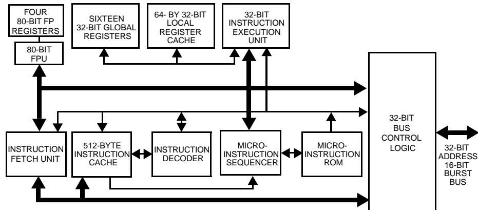
Figure 1. The 80960SB Processor's Highly Parallel Architecture
