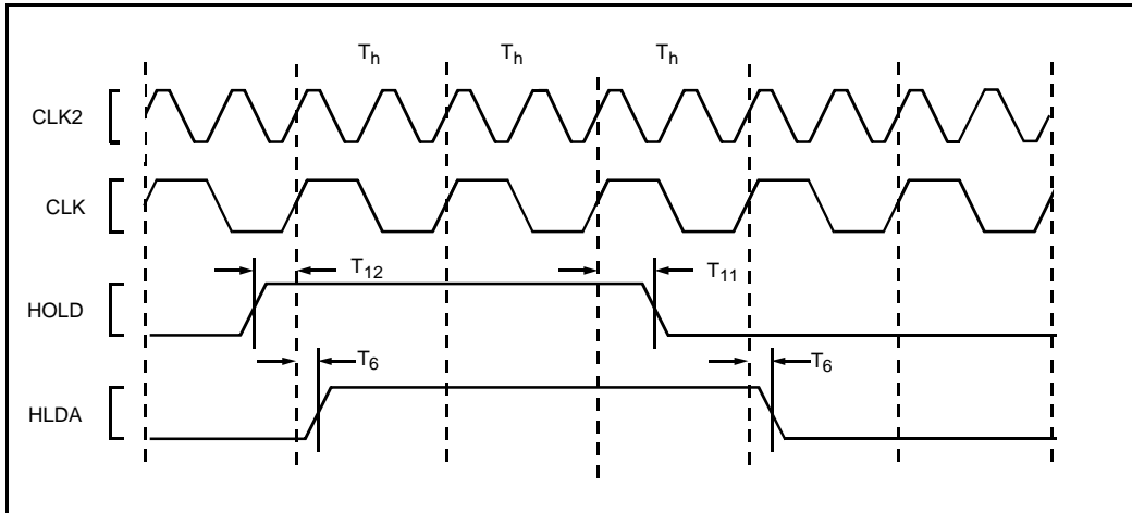
Figure 14. HOLD Timing
