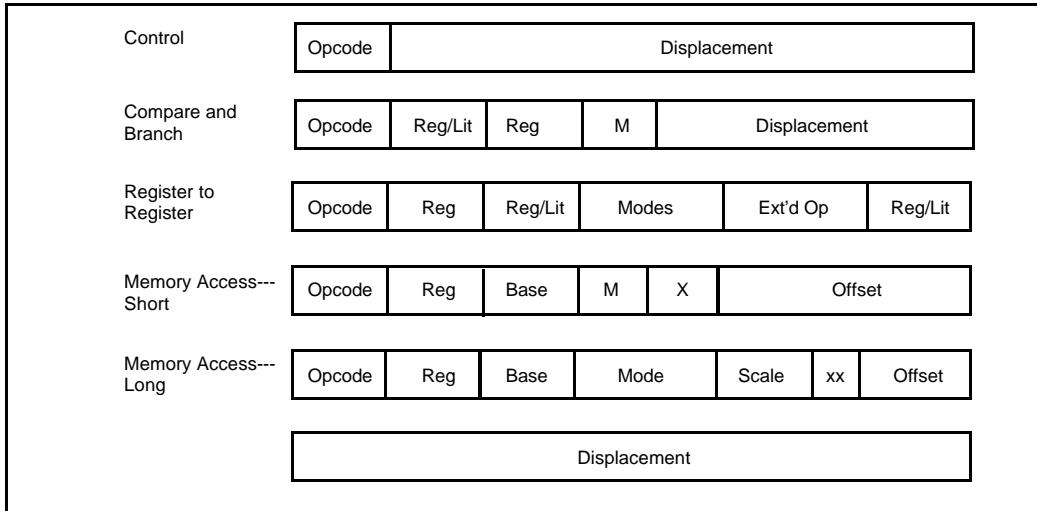
Figure 3. Instruction Formats
