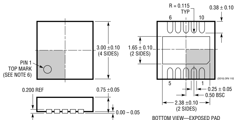
BOTTOM VIEW—EXPOSED PAD
