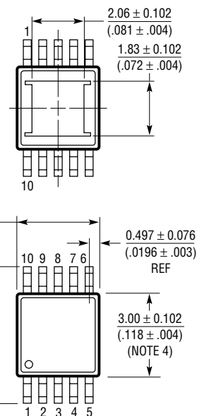
BOTTOM VIEW OF EXPOSED PAD OPTION
