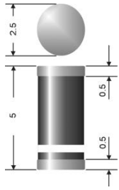
Surface mount diode
