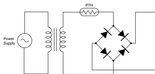
(2) Transformer Protection Circuit 2
