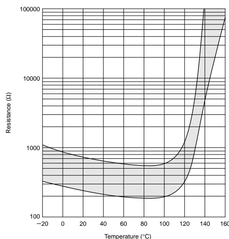
PRF_AR471Q Type
