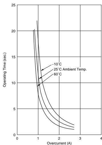
PTGL10AR3R9M3B51B0
