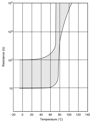
PTF_04BF471Q2N34B0
