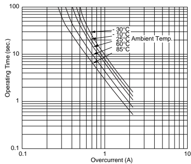
PTGL09AS7R6K6B51B0
