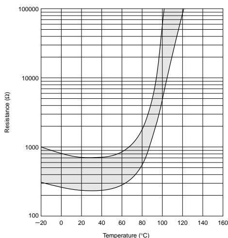
PRF_BD471Q Type
