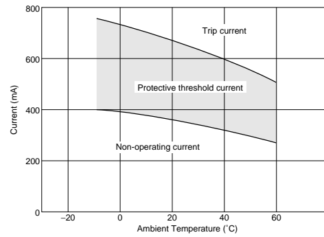
PTGL12AR5R6H4B71B0
