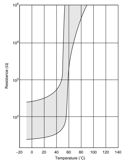
PTF_04BH222Q2N34B0
