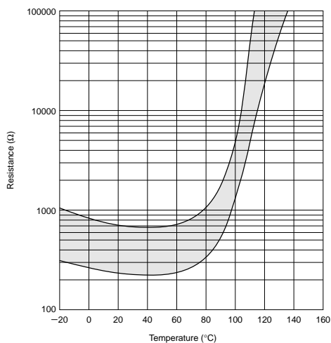
PRF_BC471Q Type
