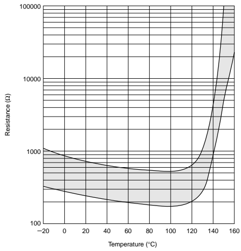
PRF_AS471Q Type
