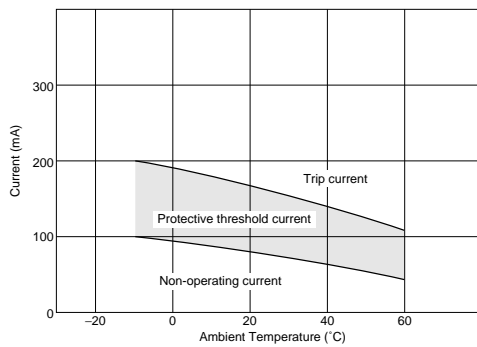
PTGL07BD220N3B51B0
