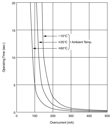
PRG21BB150MB1RK
