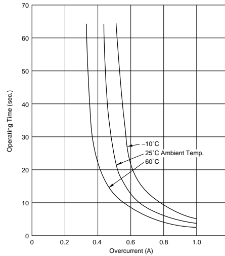
PTGL07AR4R6H2B51B0
