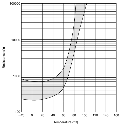
PRF_BF471Q Type
