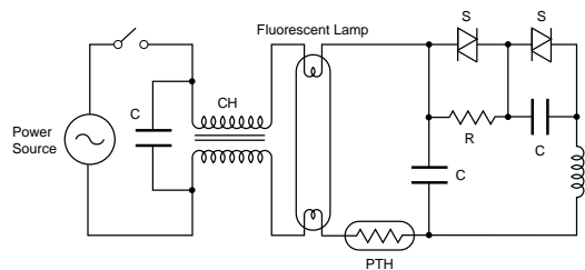
(4) Fluorescent Lamp Protection Circuit
