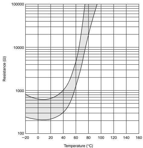
PRF_BG471Q Type
