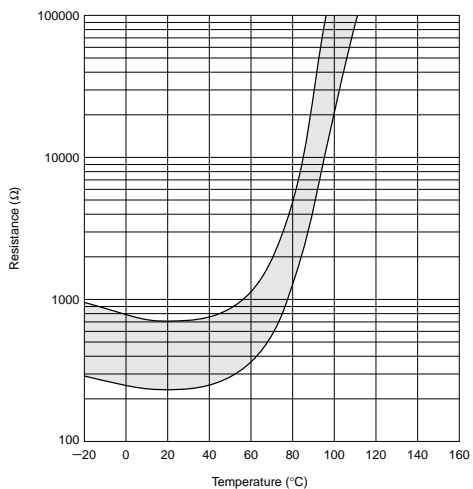
PRF_BE471Q Type
