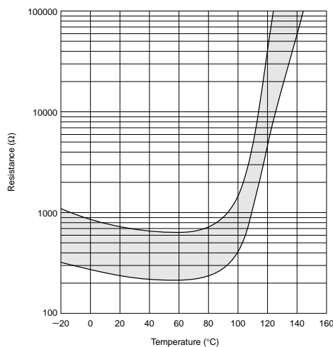
PRF_BB471Q Type
