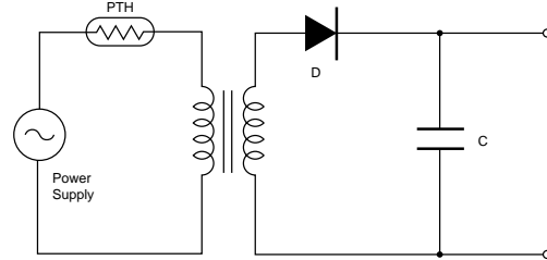
(2) Transformer Protection Circuit 1
