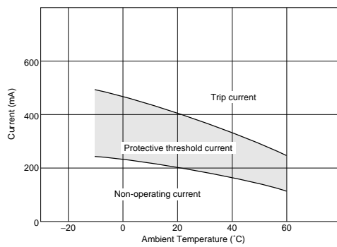
PTGL09BD4R7N2B51B0
