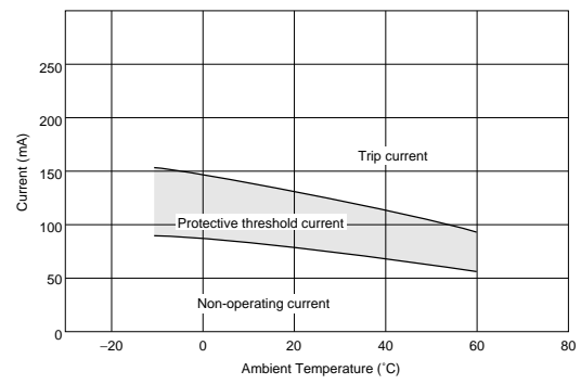
PTGL07AR820M9A51B0
