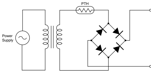
(3) Transformer Protection Circuit 2
