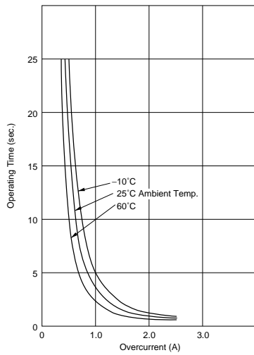
PTGL12AR270M9C01B0
