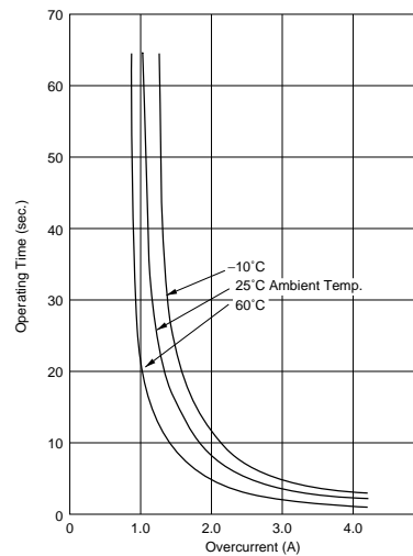
PTGL12AR1R2H2B51B0
