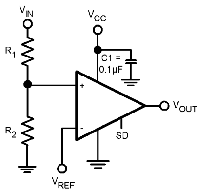
Threshold Detector
