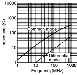
ACM2520-301-2P
