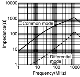
ACM3225-800-2P
