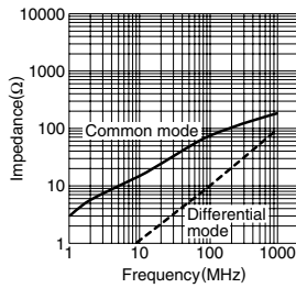
ACM3225-800-2P
