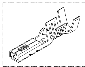
ISOMETRIC VIEW
