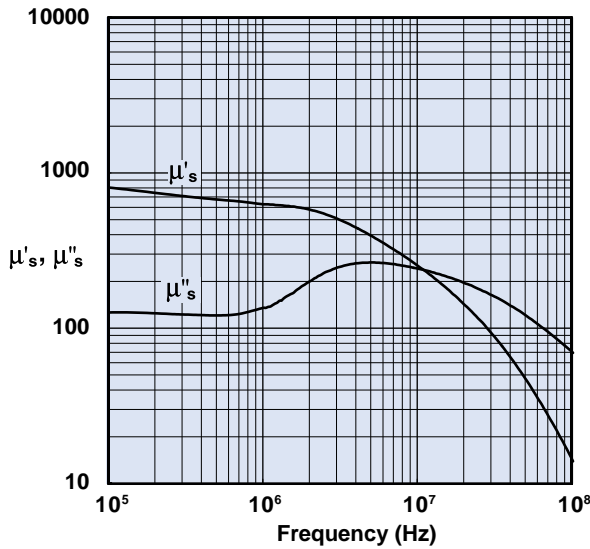
Figure 8 Complex Permeability vs. Frequency Measured on a 17/10/6mm toroid using the HP 4284A and the HP 4291A.
