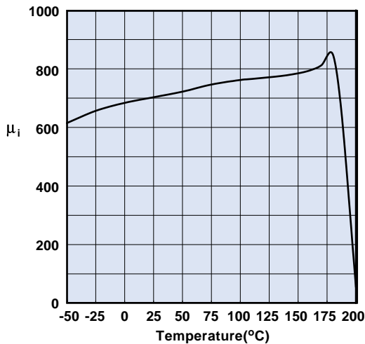
Measured on a 17/10/6mm toroid at 100kHz.
