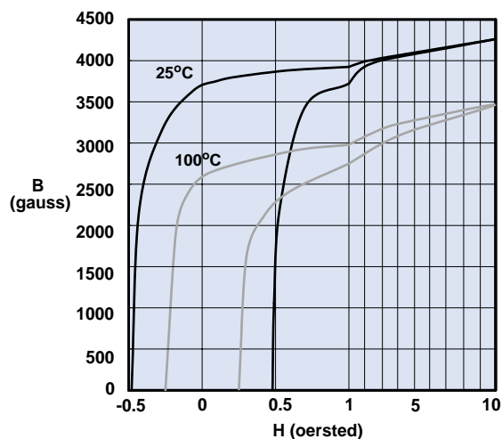
Measured on a 13/8/6mm toroid at 10 kHz.
