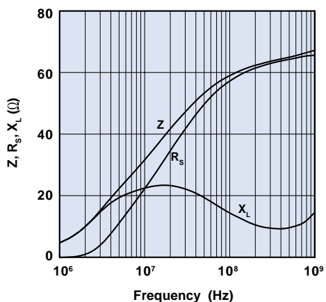
Figure 2A Impedance, reactance, and resistance vs. frequency for bead on lead 2743001112.
