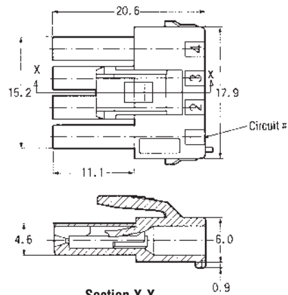
Section X-X
