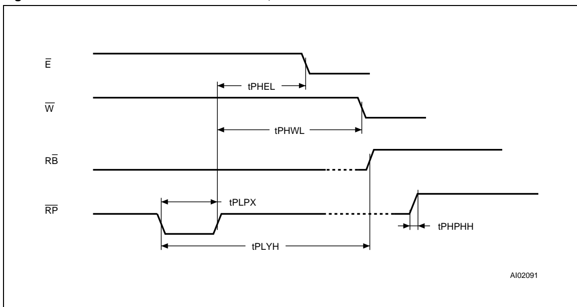
Figure 9. Read and Write AC Characteristics, \bar{R} Related
