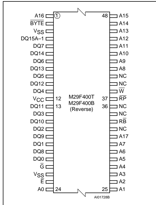
Figure 2B. TSOP Reverse Pin Connections
