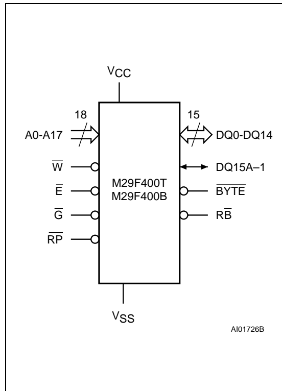
Figure 1. Logic Diagram
