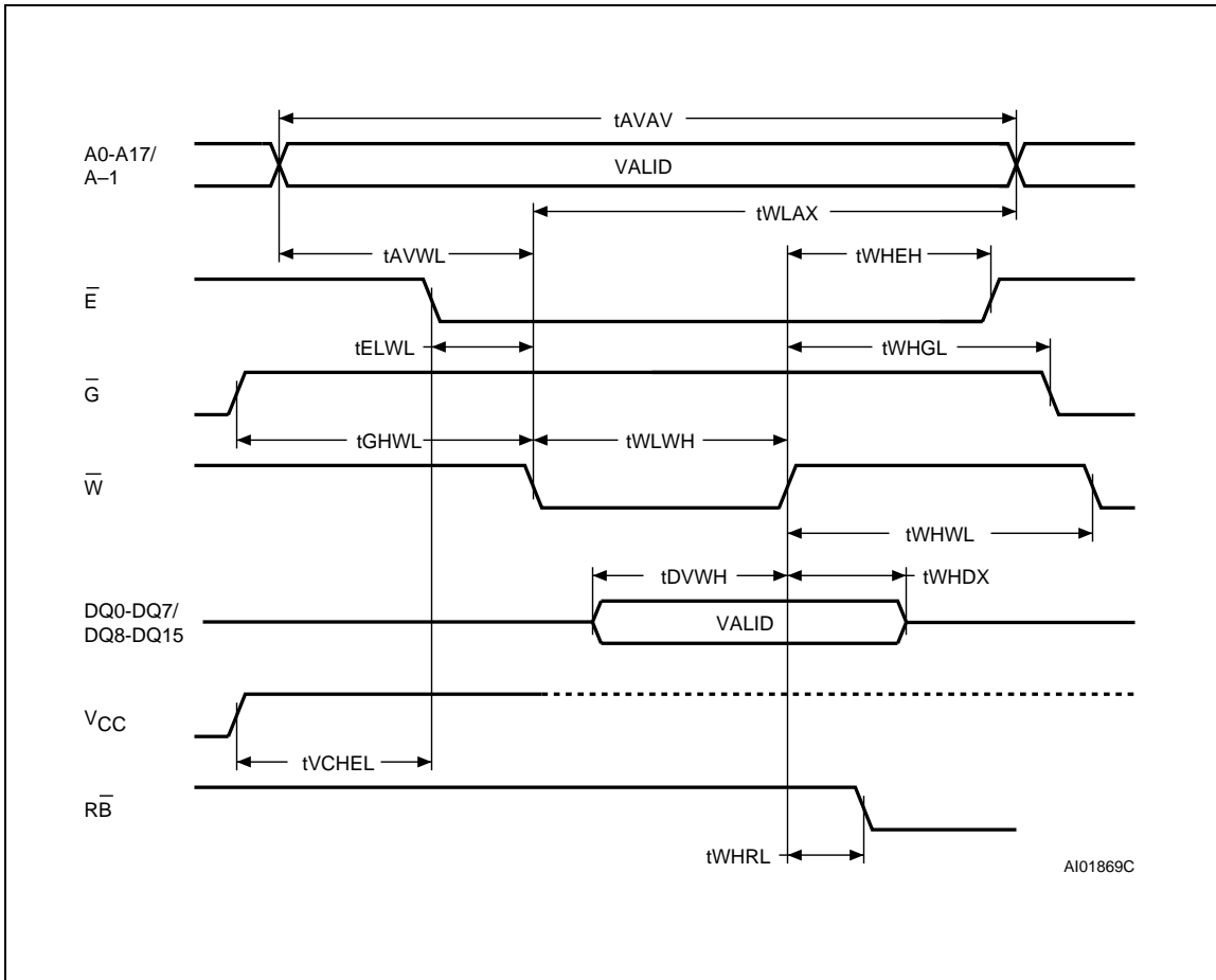
Figure 7. Write AC Waveforms, \overline{W} Controlled
