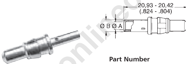
Plug
