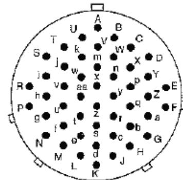
Shell Size 24 48
