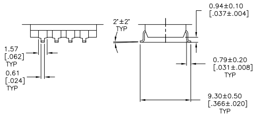
SURFACE MOUNT S (OUTSIDE "L")
