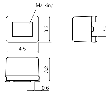
Type FB (4.5×3.2×3.2)
