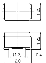
Type ND (2.0×1.25×1.25)
