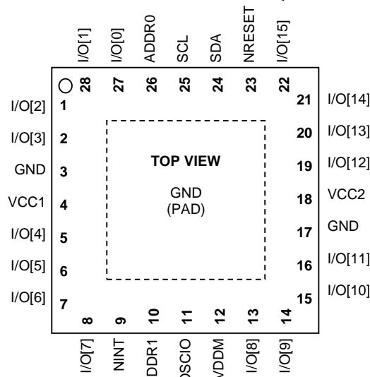
Figure 2 – SX1509 QFN-UT-28 Pinout
