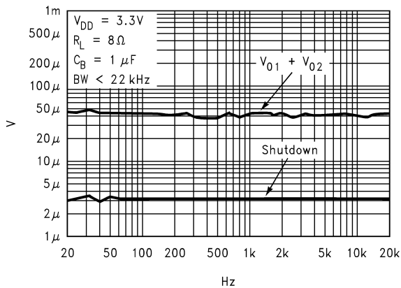
Noise Floor
