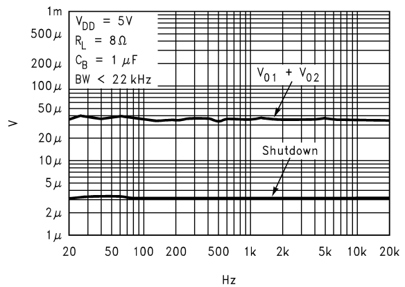
Noise Floor
