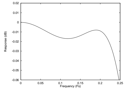
Figure 26 Digital Filter Type D Ripple
