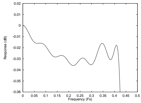
Figure 24 Digital Filter Type C Ripple
