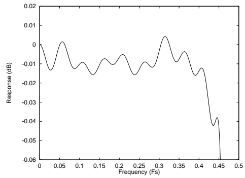
Figure 20 ADC Digital Filter Type A Ripple
