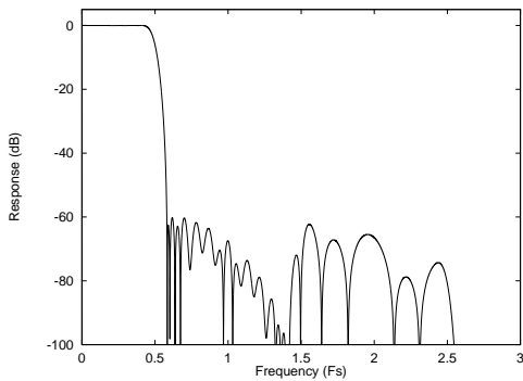
Figure 23 Digital Filter Type C Frequency Response
