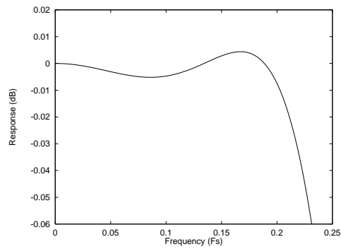
Figure 22 Digital Filter Type B Ripple
