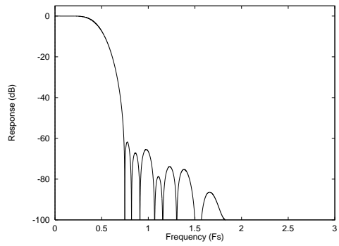
Figure 25 Digital Filter Type D Frequency Response
