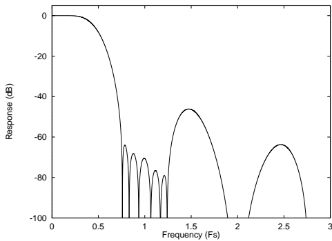
Figure 21 Digital Filter Type B Frequency Response
