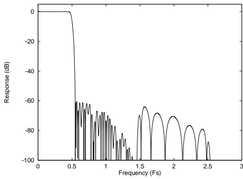
Figure 19 Digital Filter Type A Frequency Response
