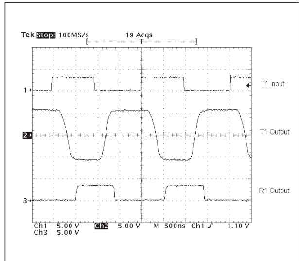
Figure 13. Driver Loopback Test One Driver 1Mbps
