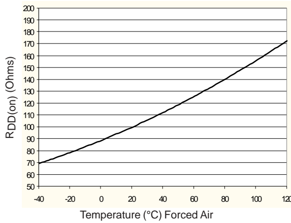
Figure 3. Typical On-Resistance
