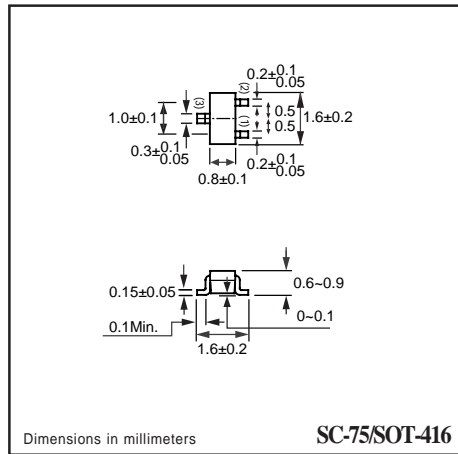
SC-75/SOT-416
