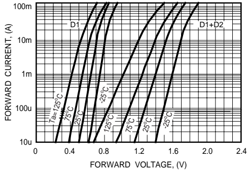
FIG. 1 - FORWARD CHARACTERISTICS
