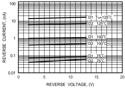
FIG. 3 - REVERSE CHARACTERISTICS
