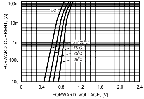
FIG. 2 - FORWARD CHARACTERISTICS
