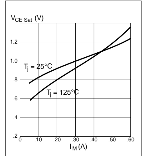
Figure 9. Typical source saturation voltage vs. output current.
