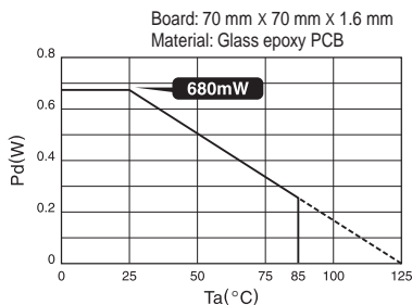
Fig. 26: HVSO6 Power Dissipation/ Power Dissipation Reduction (Example)
