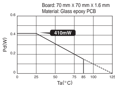
Fig. 27: HVSO5 Power Dissipation/ Power Dissipation Reduction (Example)
