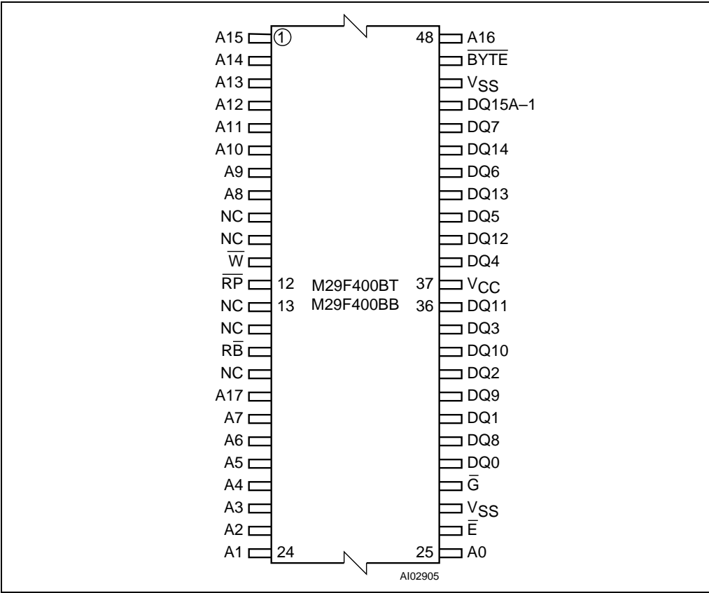
Figure 2. TSOP connections
