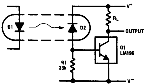
Fast Optically Isolated Switch
