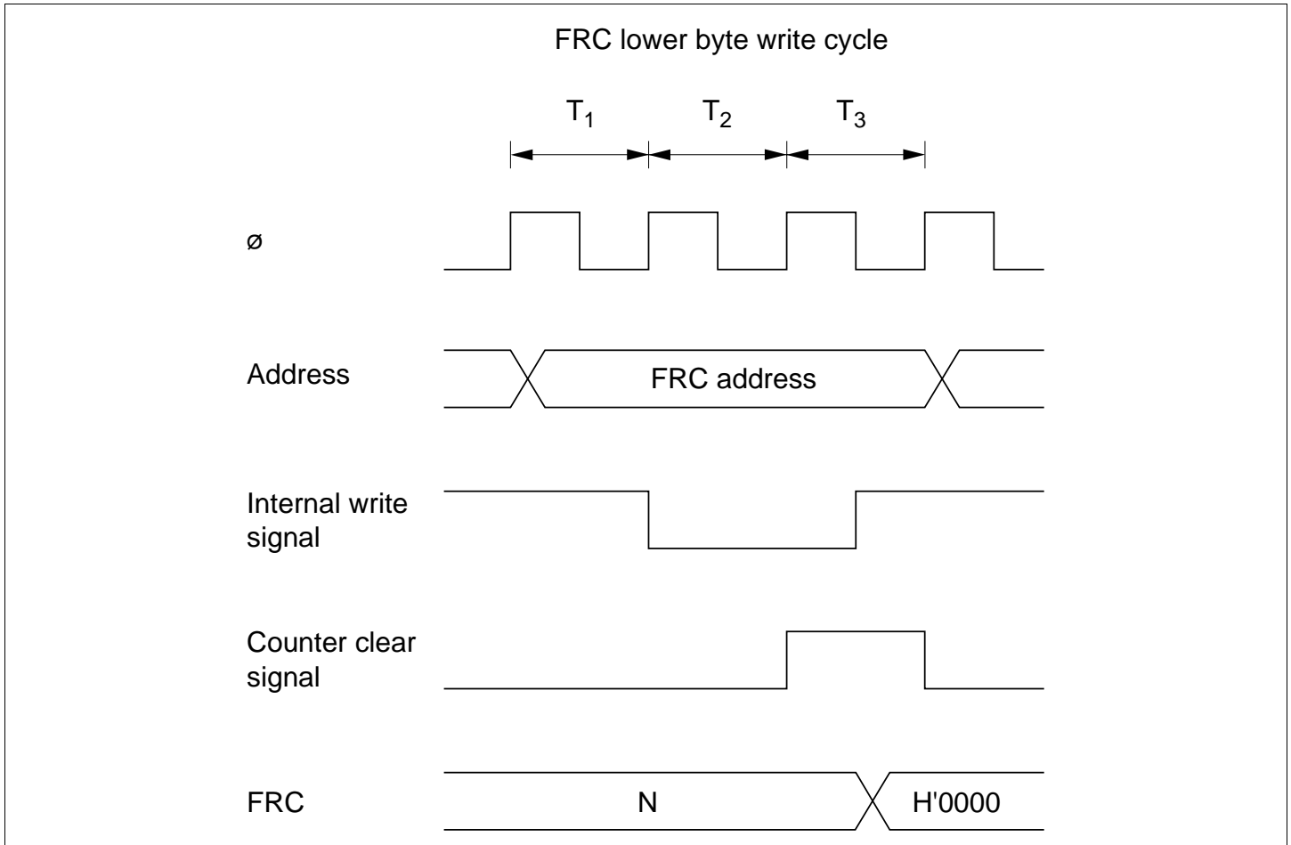
Figure 9.32 Contention between FRC Write and Clear
