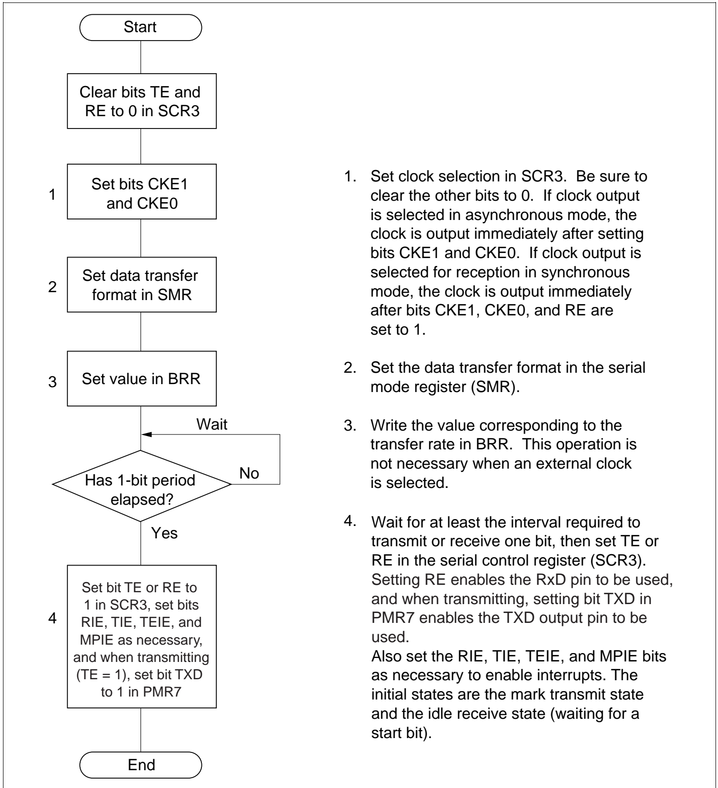
Figure 10.10 Example of SCI3 Initialization Flowchart
