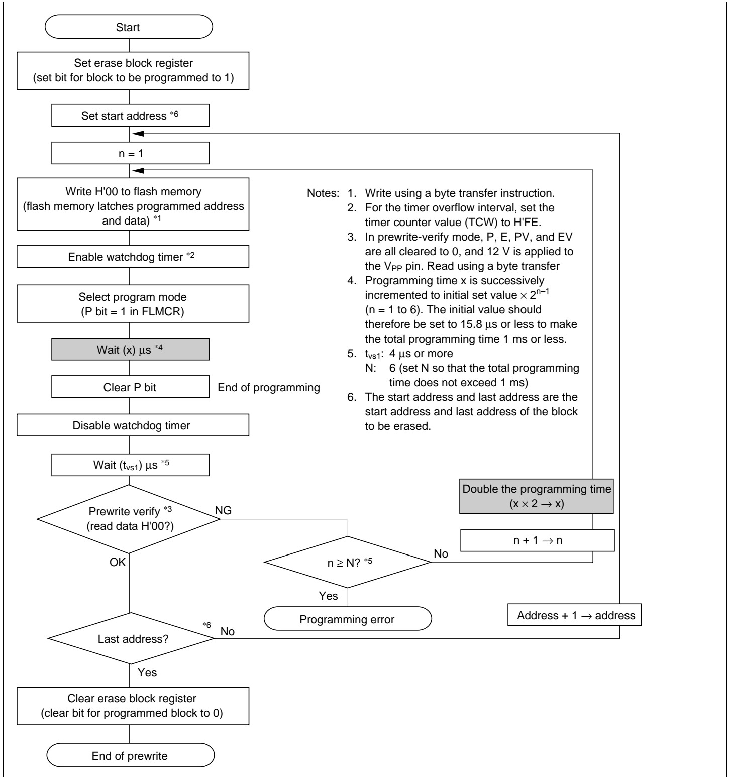
Figure 6.16 Prewrite Flowchart
