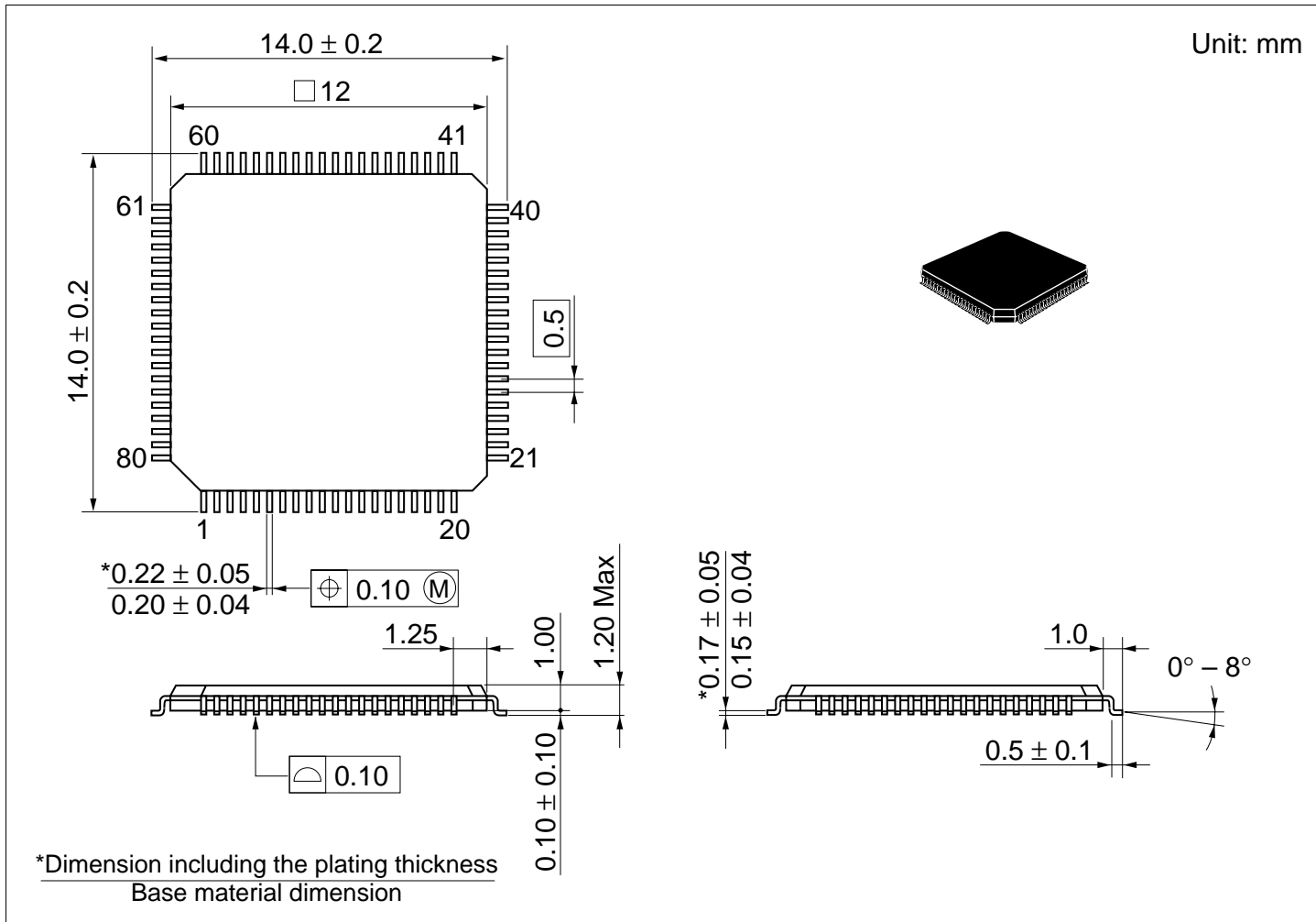
Figure F.3 TFP-80C Package Dimensions
