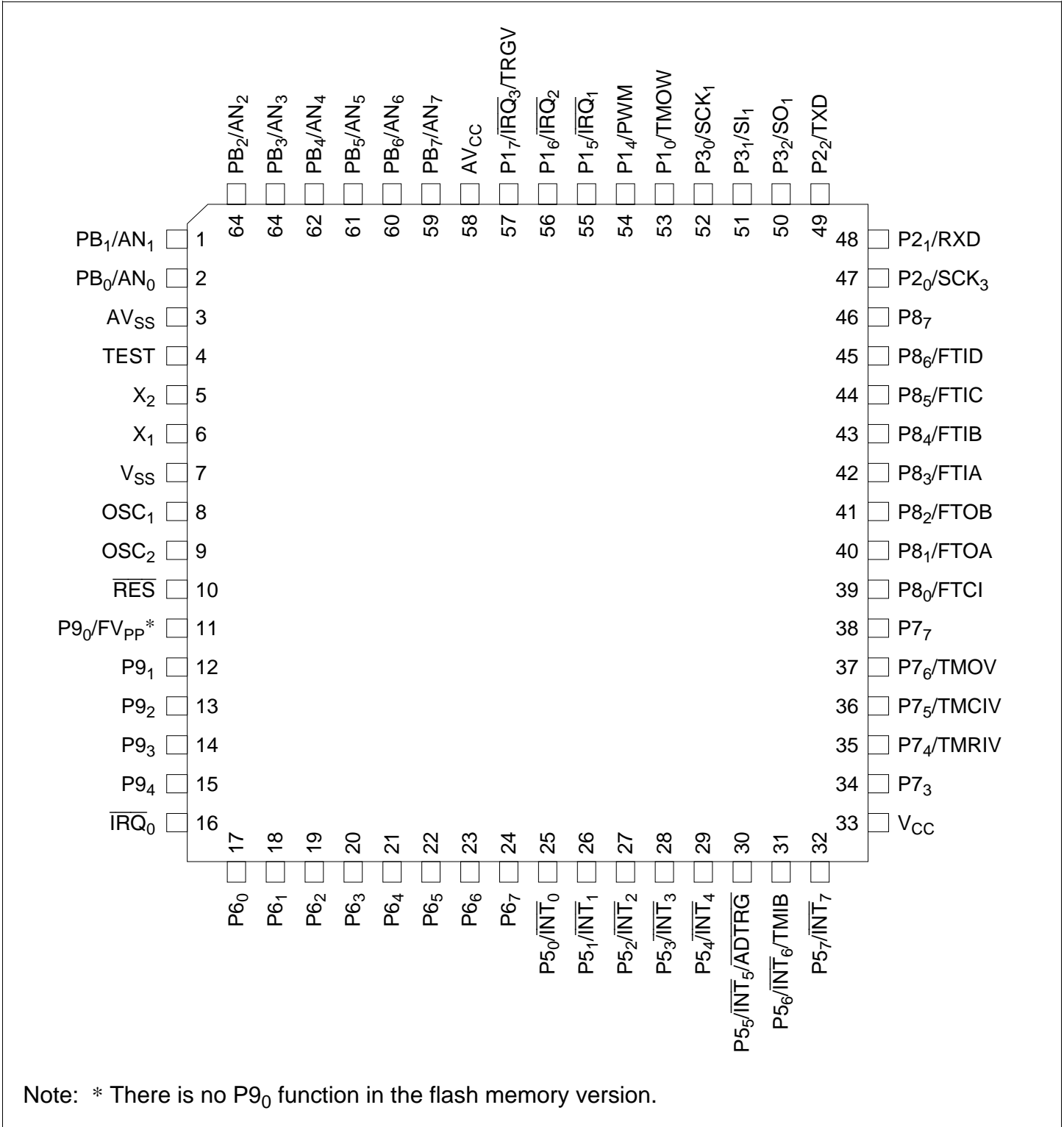
Figure 1.2 Pin Arrangement (FP-64A: Top View)
