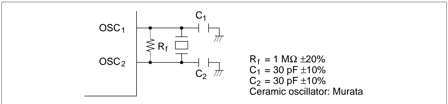
Figure 4.4 Typical Connection to Ceramic Oscillator
