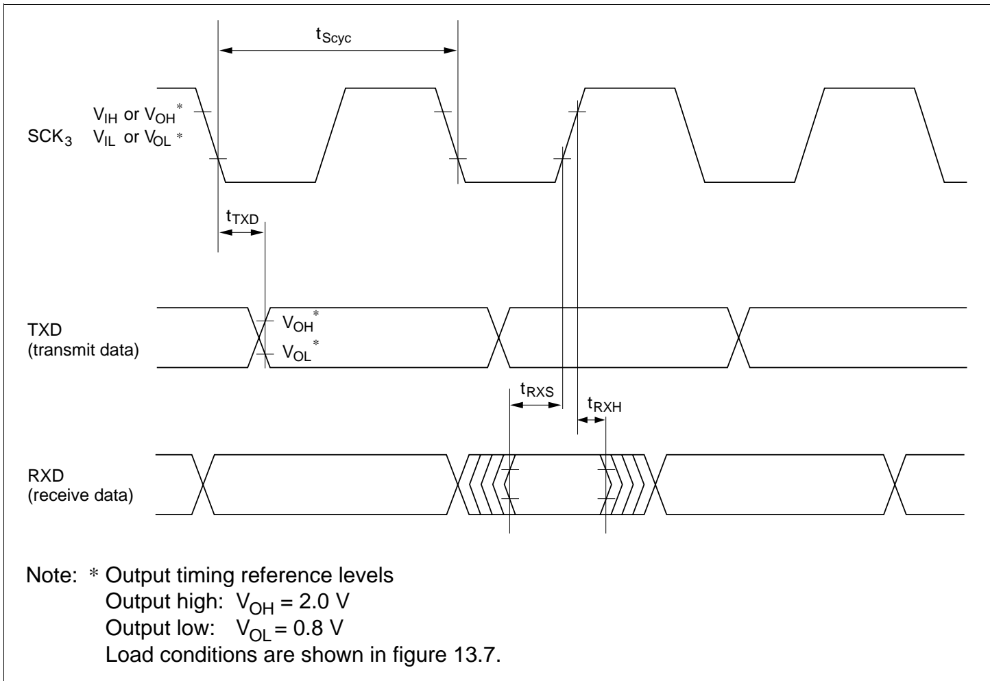
Figure 13.6 Serial Interface 3 Synchronous Mode Input/Output Timing
