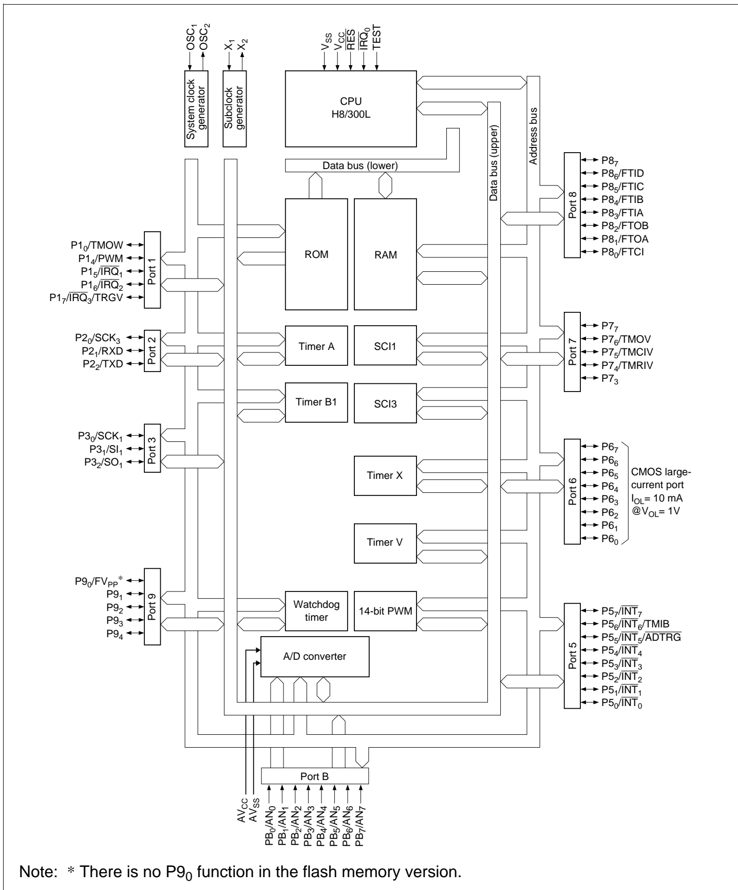
Figure 1.1 Block Diagram
