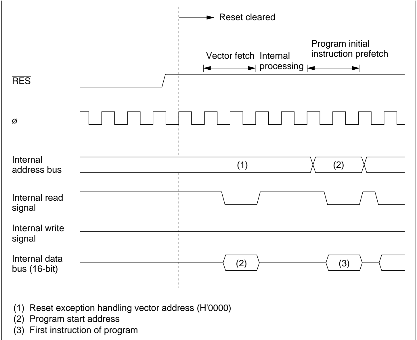
Figure 3.1 Reset Sequence
