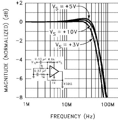
Frequency Response for Various Supply Voltages, A_V = +2
