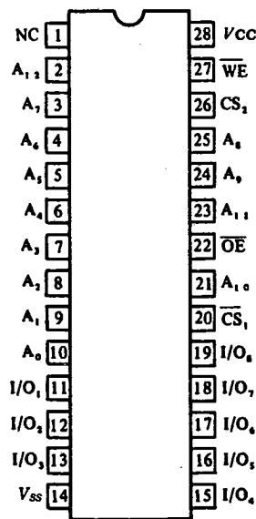
(Top View)
