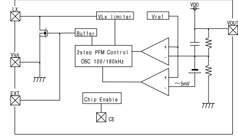
(1) XC6383A~XC6383D (VOUT端与VDD共用)
