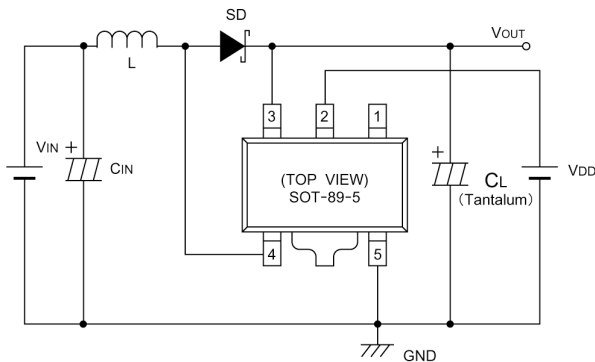
Circuit 3: XC6372E series
