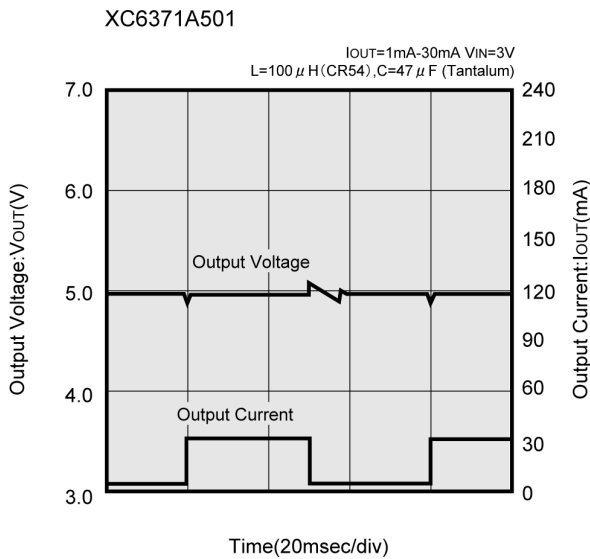
(6) Load Transient Response
