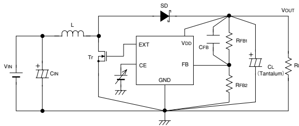
Circuit 3. XC6367C, XC6368C
