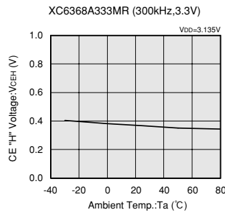
(19) CE "H" VOLTAGE vs. AMBIENT TEMPERATURE
