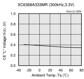
(18) CE "L" VOLTAGE vs. AMBIENT TEMPERATURE
