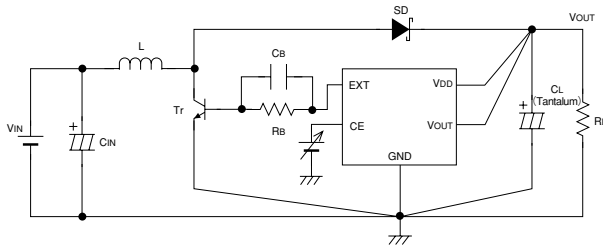
Circuit 8. XC6367B, XC6368B (NPN Transistor)
