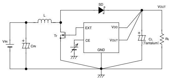
Circuit 2. XC6367B, XC6368B
