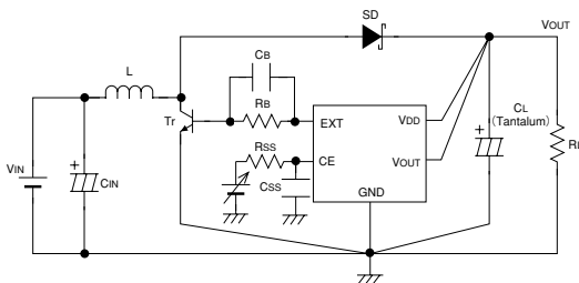
Circuit 9. XC6367C, XC6368C (NPN Transistor)
