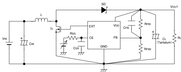
Circuit 5. XC6367E, XC6368E
