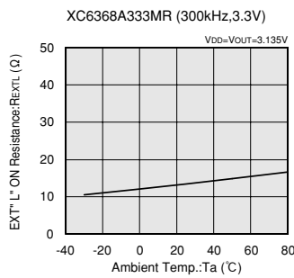
(9) EXT L ON RESISTANCE vs. AMBIENT TEMPERATURE
