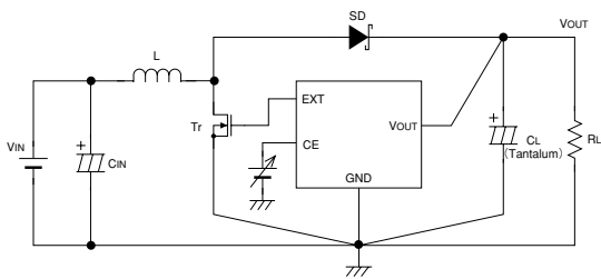
Circuit 5. XC6367E, XC6368E
