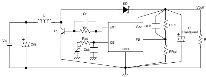
Circuit 10. XC6367D, XC6368D (NPN Transistor)
