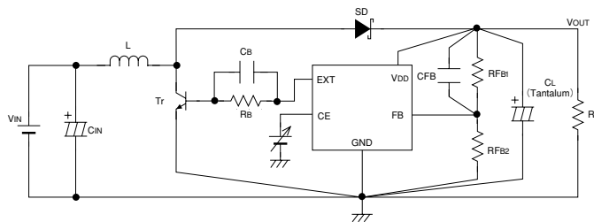
Circuit 9. XC6367C, XC6368C (NPN Transistor)
