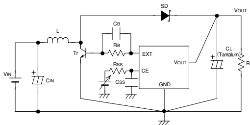
Circuit 12. XC6367F, XC6368F (NPN Transistor)
