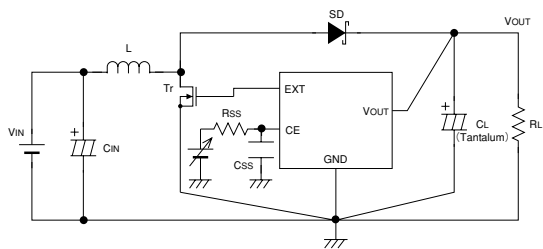
Circuit 6. XC6367F, XC6368F
