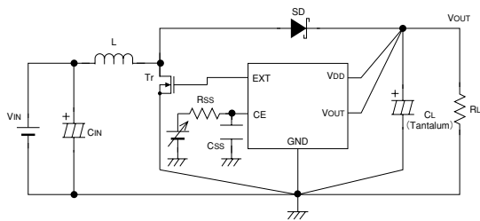
Circuit 3. XC6367C, XC6368C
