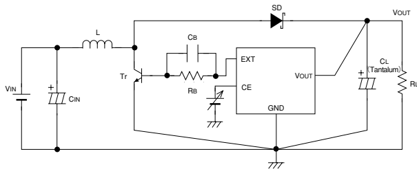
Circuit 12. XC6367F, XC6368F (NPN Transistor)
