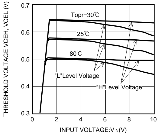
XC62HR5002 (5V)
