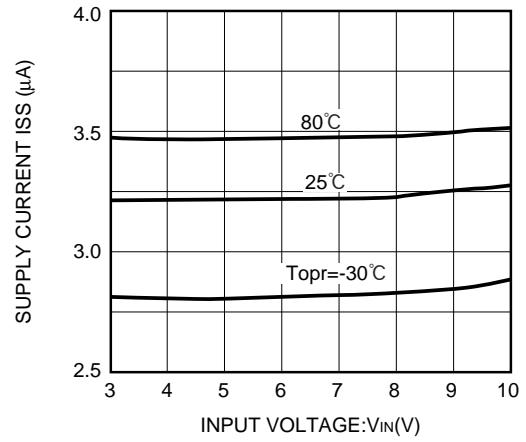
XC62HR3002 (3V)
