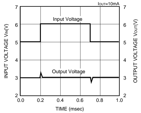
XC62HR3002 (3V)
