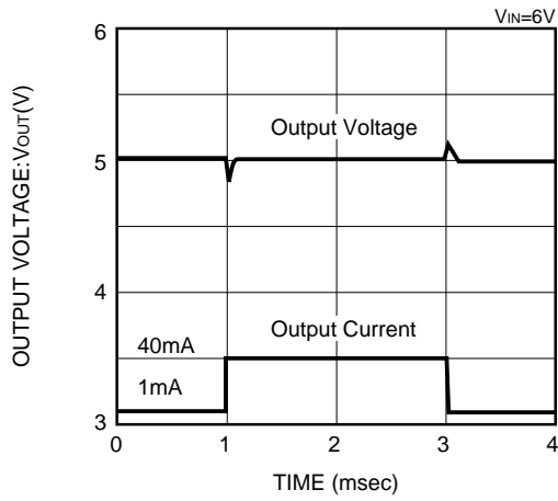
XC62HR5002 (5V)
