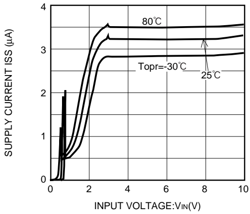
XC62HR3002 (3V)
