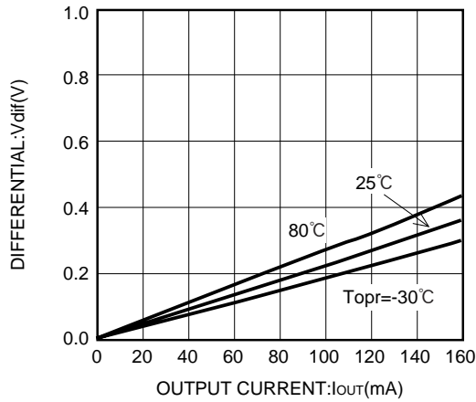
XC62HR5002 (5V)
