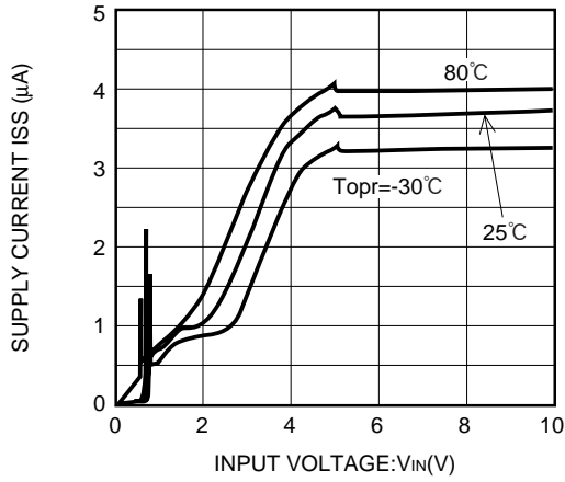
XC62HR5002 (5V)
