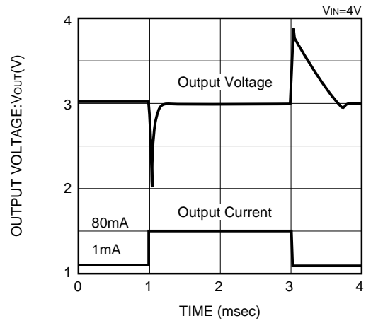
XC62HR3002 (3V)
