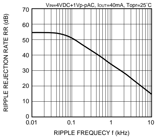
XC62HR3002
