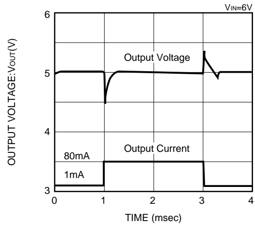
XC62HR5002 (5V)
