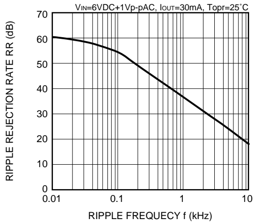
XC62HR5002
