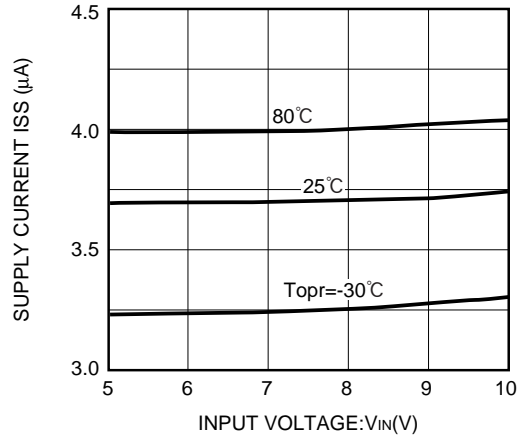
XC62HR5002 (5V)
