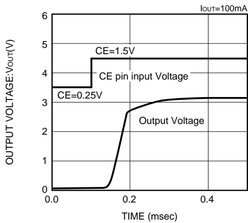
XC62HR3002 (3V)
