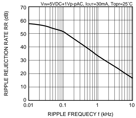
XC62HR4002
