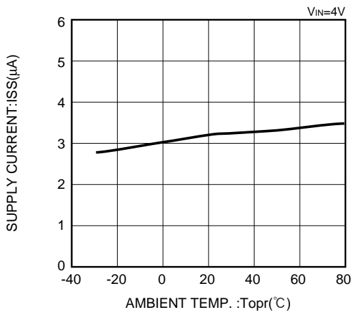
XC62HR3002 (3V)
