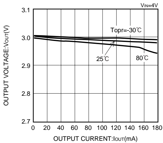
XC62HR3002 (3V)
