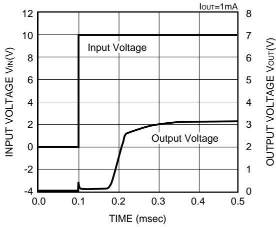
XC62HR3002 (3V)
