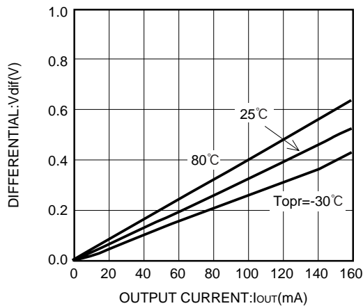
XC62HR3002 (3V)
