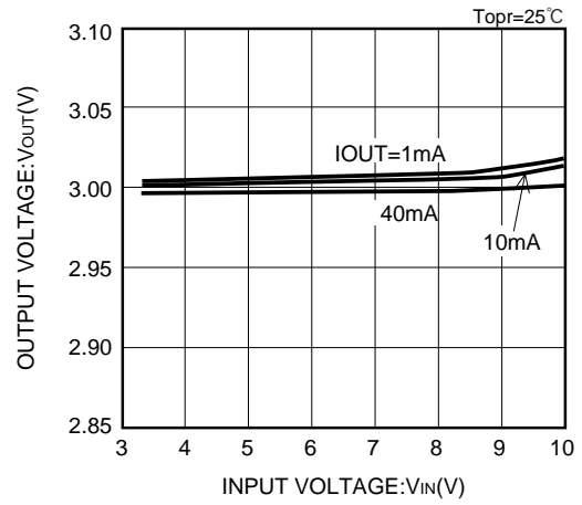
XC62HR3002 (3V)
