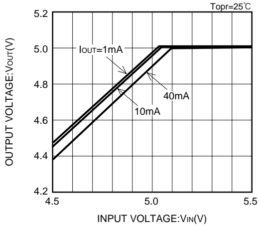
XC62HR5002 (5V)
