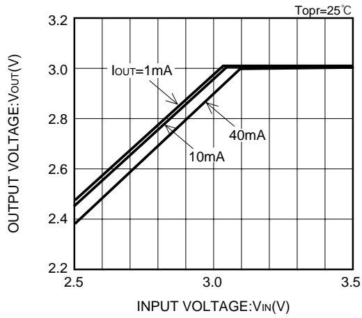
XC62HR3002 (3V)
