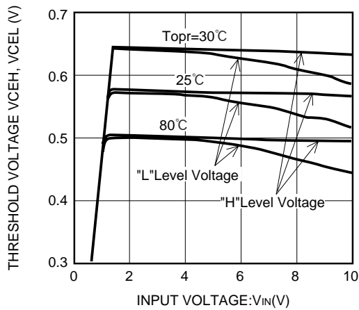
XC62HR3002 (3V)
