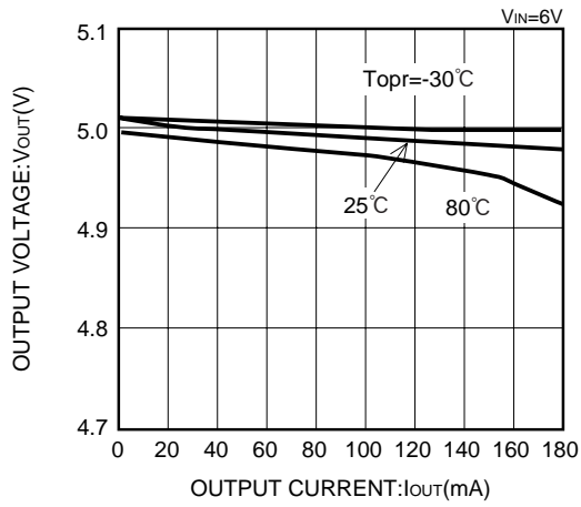
XC62HR5002 (5V)
