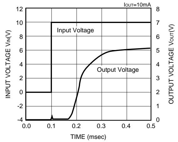
XC62HR5002 (5V)
