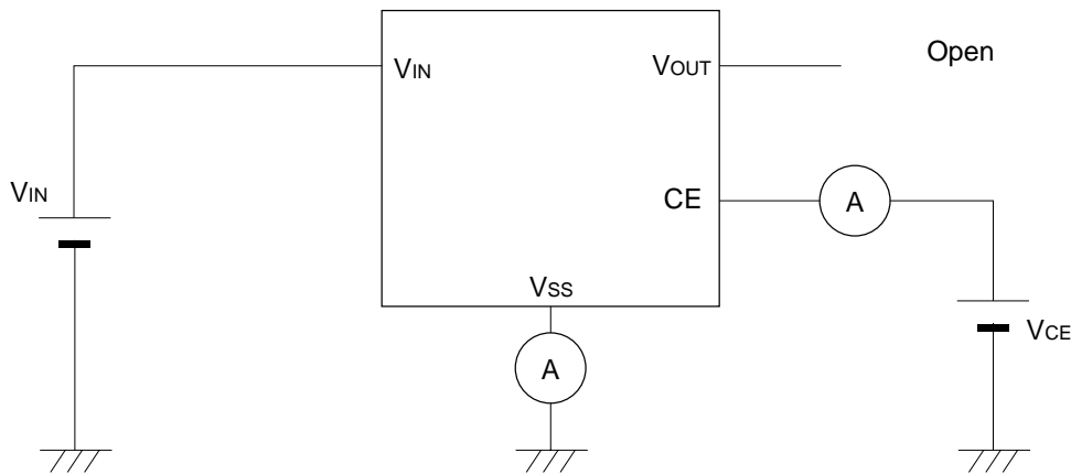
Circuit 2
