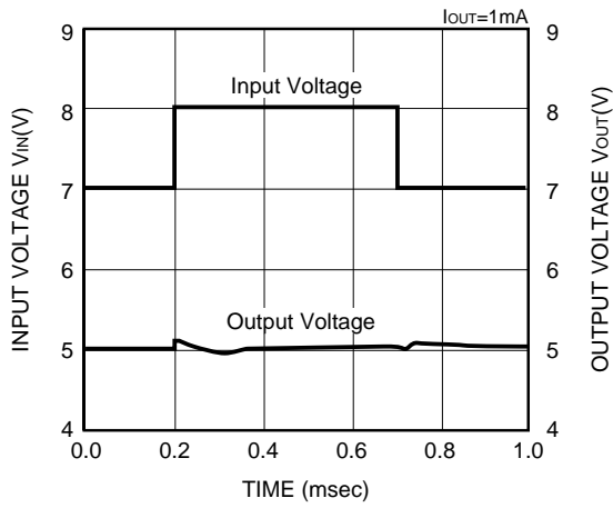
XC62HR5002 (5V)
