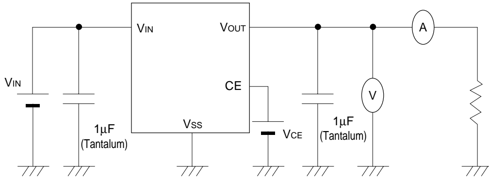
Circuit 1
