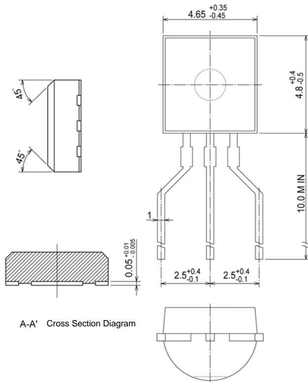
TO-92
