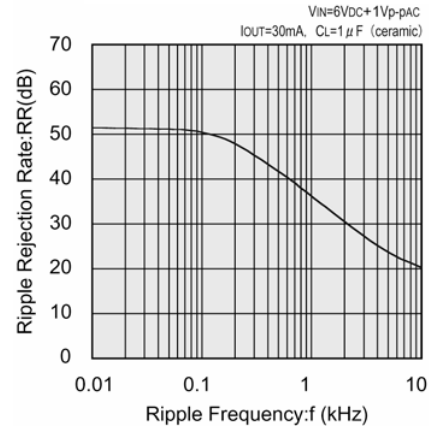
XC6202P502 (5.0V)
