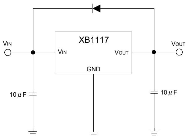
Regulator with reverse diode protection
