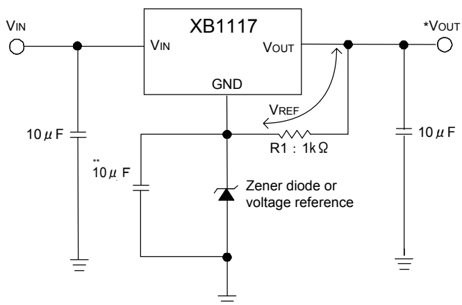
Regulator with reference voltage
