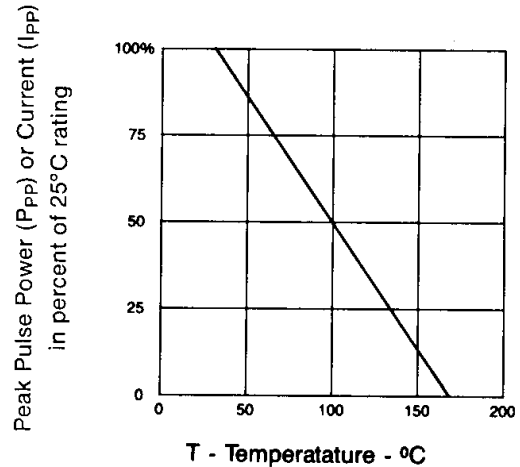
FIGURE 3 DERATING CURVE
