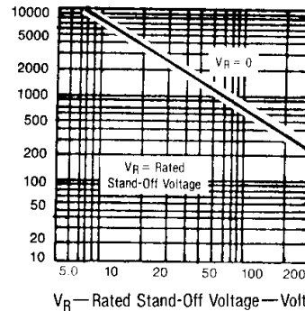
FIGURE 4 TYPICAL CAPACITANCE VS STAND-OFF VOLTAGE
