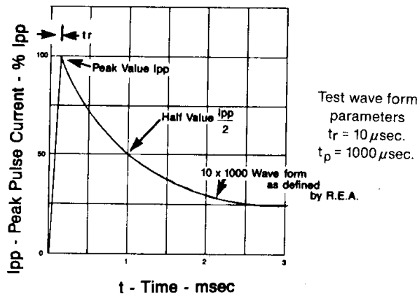
FIGURE 2 PULSE WAVEFORM
