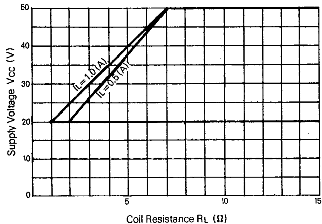
SI-7200E Operating Voltage Range
