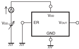
I/O characteristic
