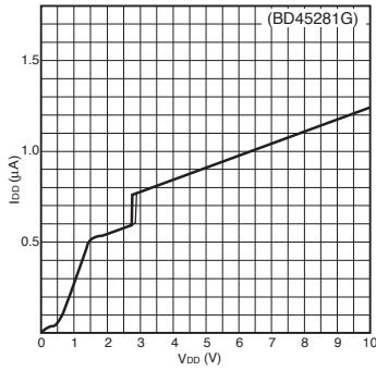
Circuit current
