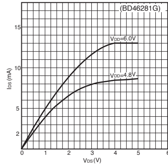
"H" output current
