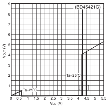
I/O characteristic
