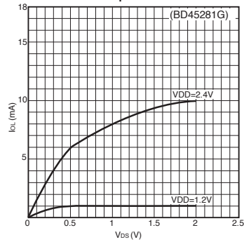
"L" output current
