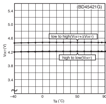
Detection voltage
