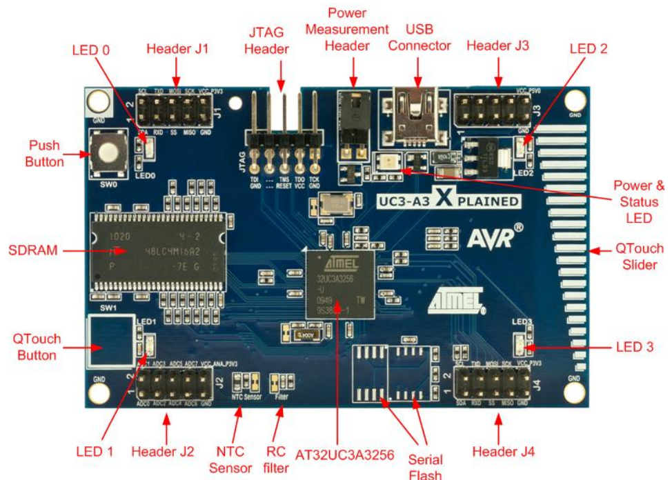
Figure 3-1. Overview of the UC3-A3 XPLAINED kit.
