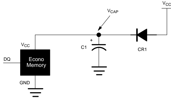
SUGGESTED CIRCUIT Figure 9
