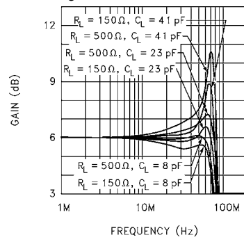
EL4431 Frequency Response for Various RL, CL VS = ±15V
