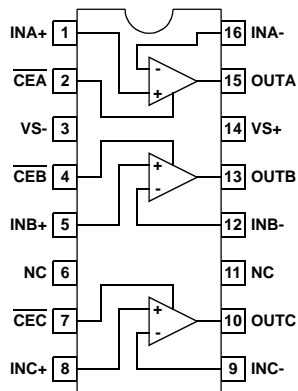
EL5392 [16-PIN SO (0.150") & QSOP] TOP VIEW
