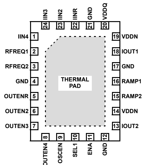
EL6838 (24-PIN LPP) TOP VIEW
