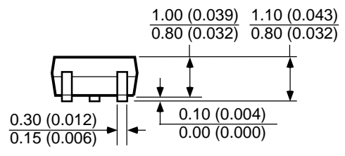
SC-70-5 (C5)
