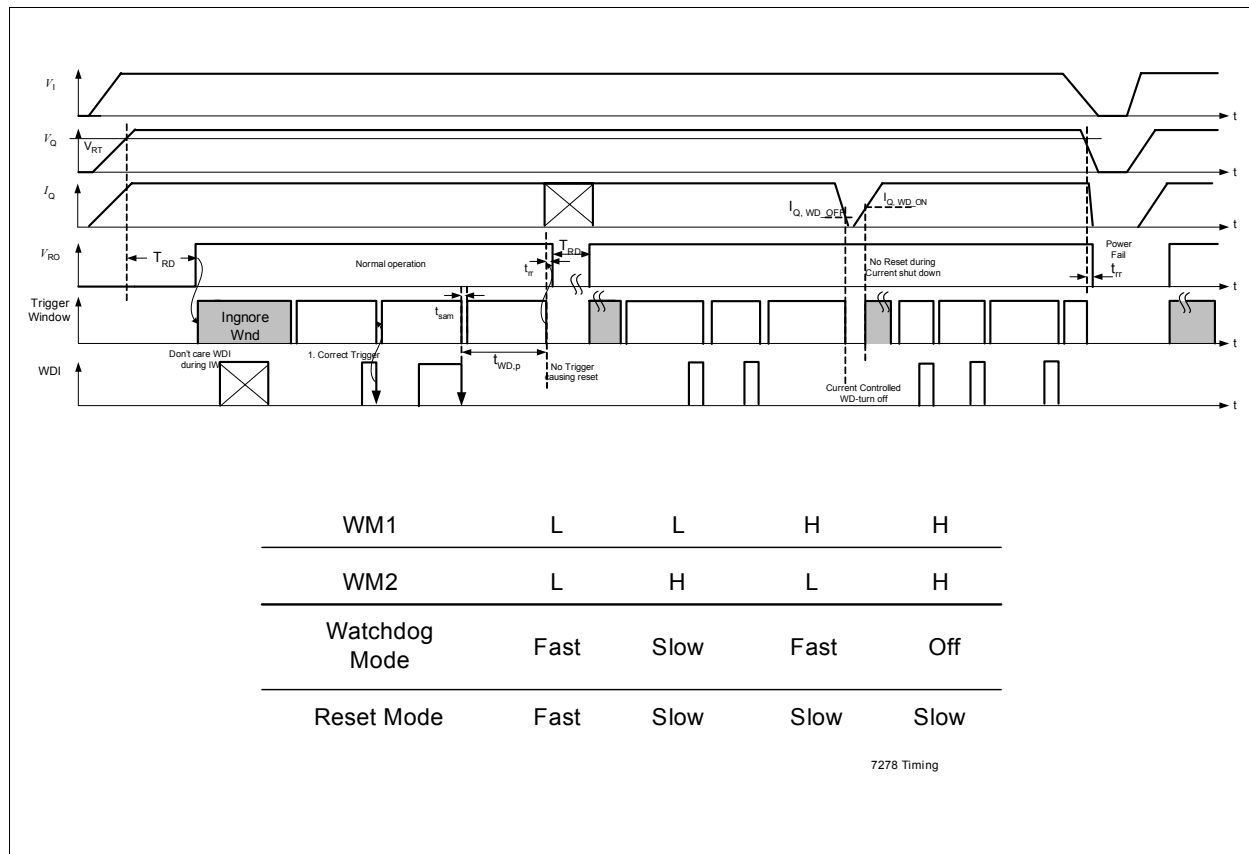
Figure 5 Watchdog Timing Diagram, Watchdog and Reset Modes
