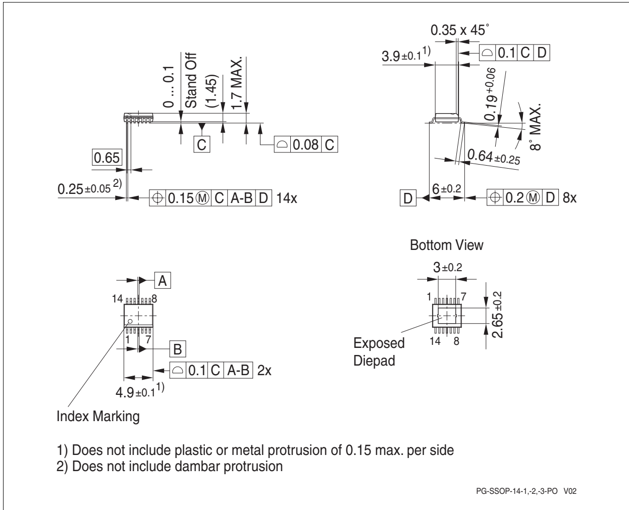
Figure 7 PG-SSOP-14 Exposed Pad
