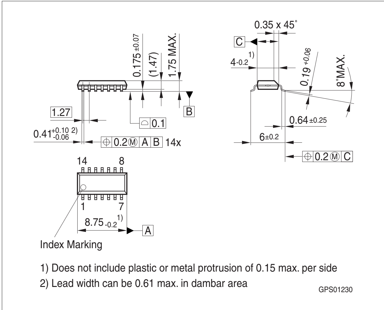
Figure 6 PG-DSO-14 (Plastic/Plastic Green - Dual Small Outline Package)
