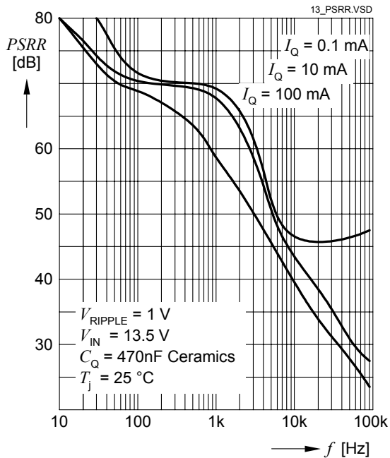
Power Supply Ripple Rejection PSRR
