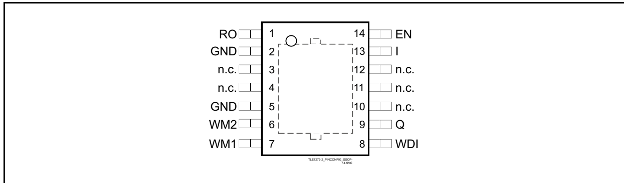
Figure 3 Pin Assignment PG-SSOP-14 Exposed Pad (top view)
