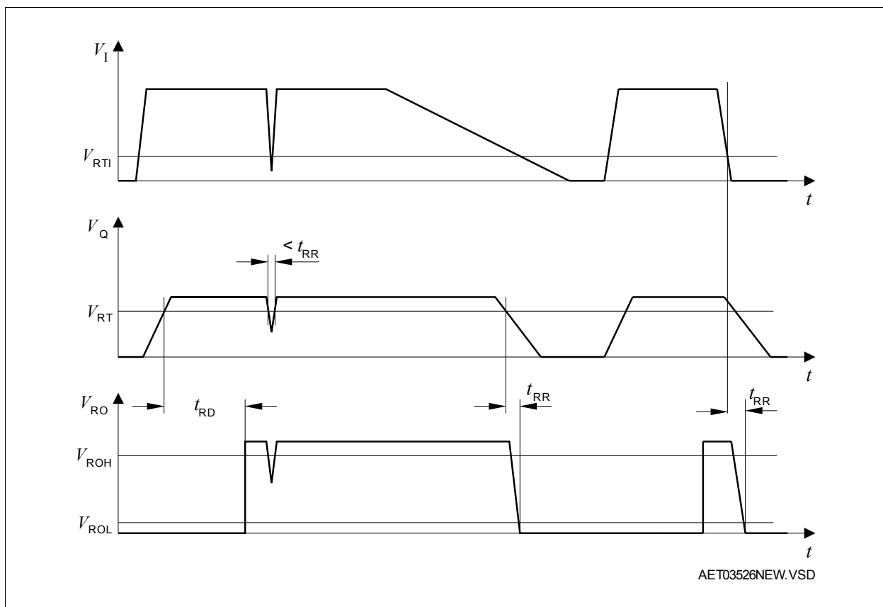
Figure 4 Reset Function and Timing Diagram
