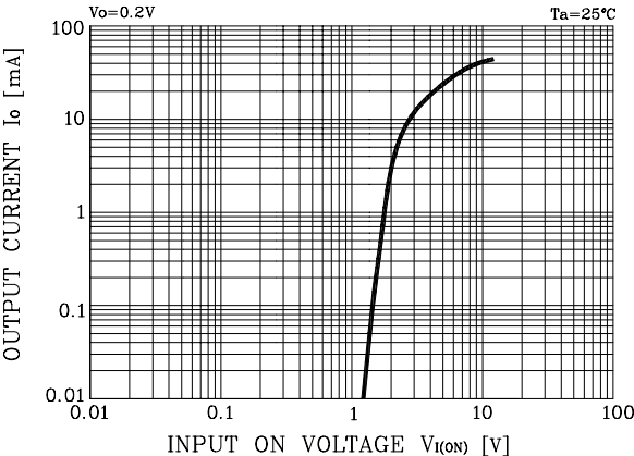
Fig. 1 I_O - V_{I(ON)}
