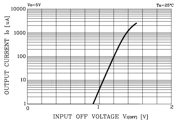
Fig. 2 I_O - V_{I(OFF)}
