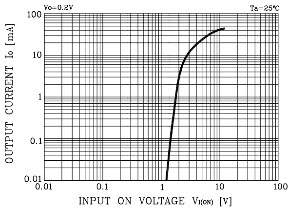
Fig. 1 I_O - V_{I(ON)}
