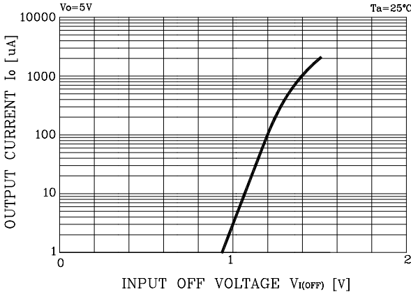
Fig. 2 I_O - V_{I(OFF)}
