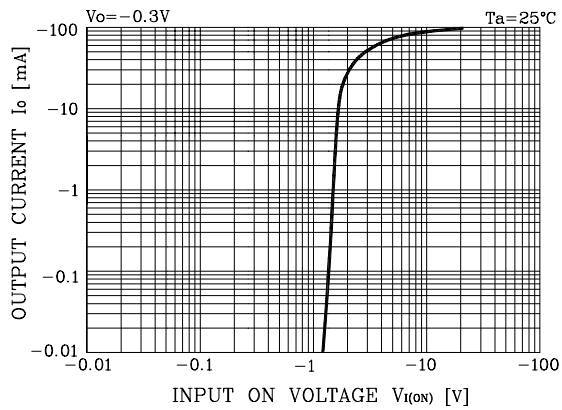
Fig. 1 I_O - V_{I(ON)}
