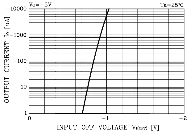
Fig. 2 I_O - V_{I(OFF)}
