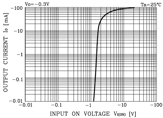
Fig. 1 I_O - V_{I(ON)}
