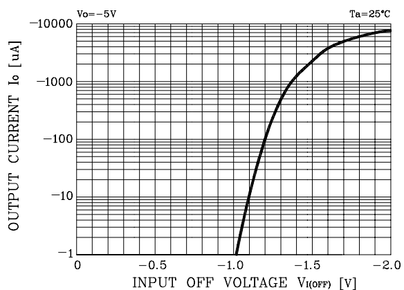
Fig. 2 I_O - V_{I(OFF)}
